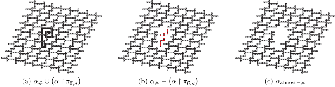
Figure 9: The black tiles are the path \pi_{\vec{0}, \vec{a}} . Since \alpha_{\#} - (\alpha \upharpoonright \pi_{\vec{0}, \vec{a}}) may have a finite number of disconnected “islands”, we remove these as well to get the largest connected subassembly of \alpha_{\#} .
