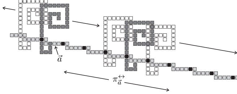
Figure 6: An example of the conclusion of Lemma 4.8. Note that the path \pi_{\vec{a}}^{\leftrightarrow} is a (two-way infinite) \vec{v} -periodic path, which means that (copies of) the path \pi_{\vec{0}, \vec{a}} can be translated in the \pm\vec{v} direction.
