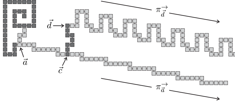
Figure 5: An example of the hypothesis of Lemma 4.8. The seed tile is at the center of the “spiral.” The path \pi_{\vec{c}, \vec{d}} is represented by the dark tiles that form the “bridge” between the tail of \pi_{\vec{a}}^{\rightarrow} (the lowest \vec{v} -periodic path) and some point on \pi_{\vec{d}}^{\rightarrow} (the upper \vec{v} -periodic path).
